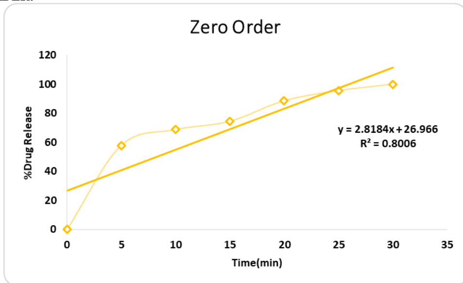
Figure No:8 Zero order plot of Roflumilast F12 Formulation
