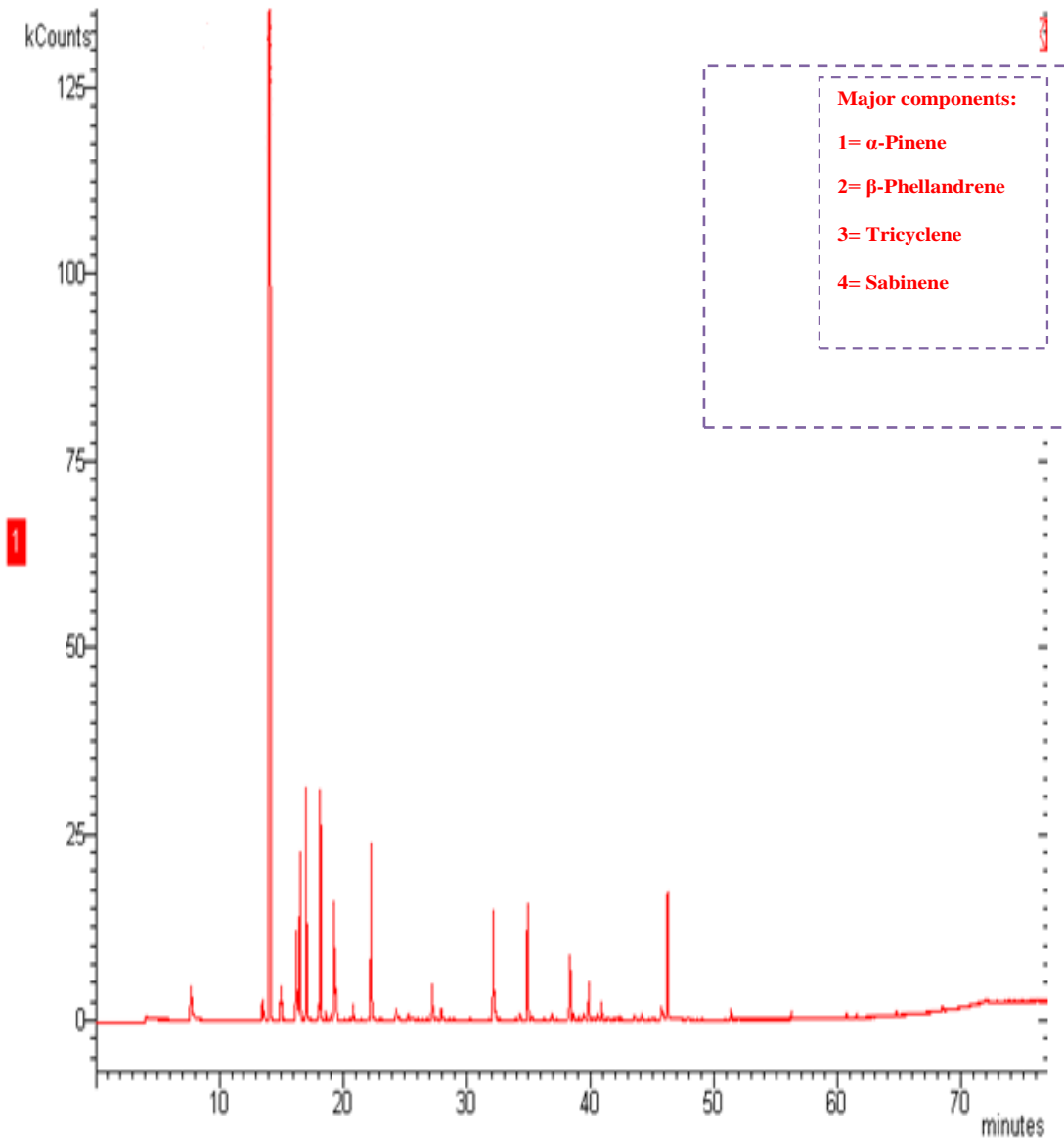
FIG: 1 Order of elution of various constituents of analysed essential oil
