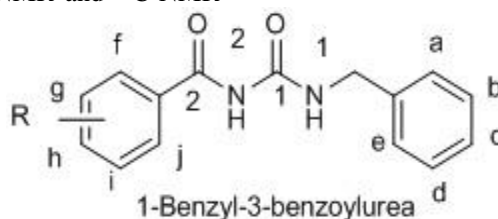
Figure 1 : The structure of 1-benzyl-3-benzoylurea (R = H)
